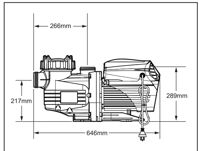
Figure 2. Side Dimensions
