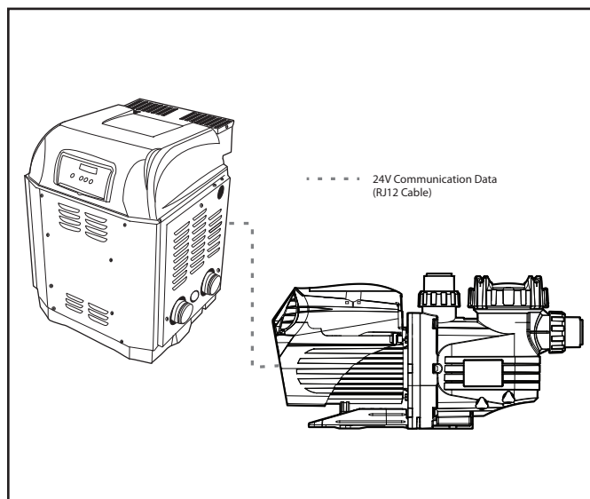
Figure 29. Viron XT Series 2 Pump with RJ12 Cable Connection
