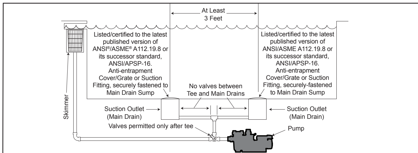
Figure 9. Number of Suction Outlets Per Pump
