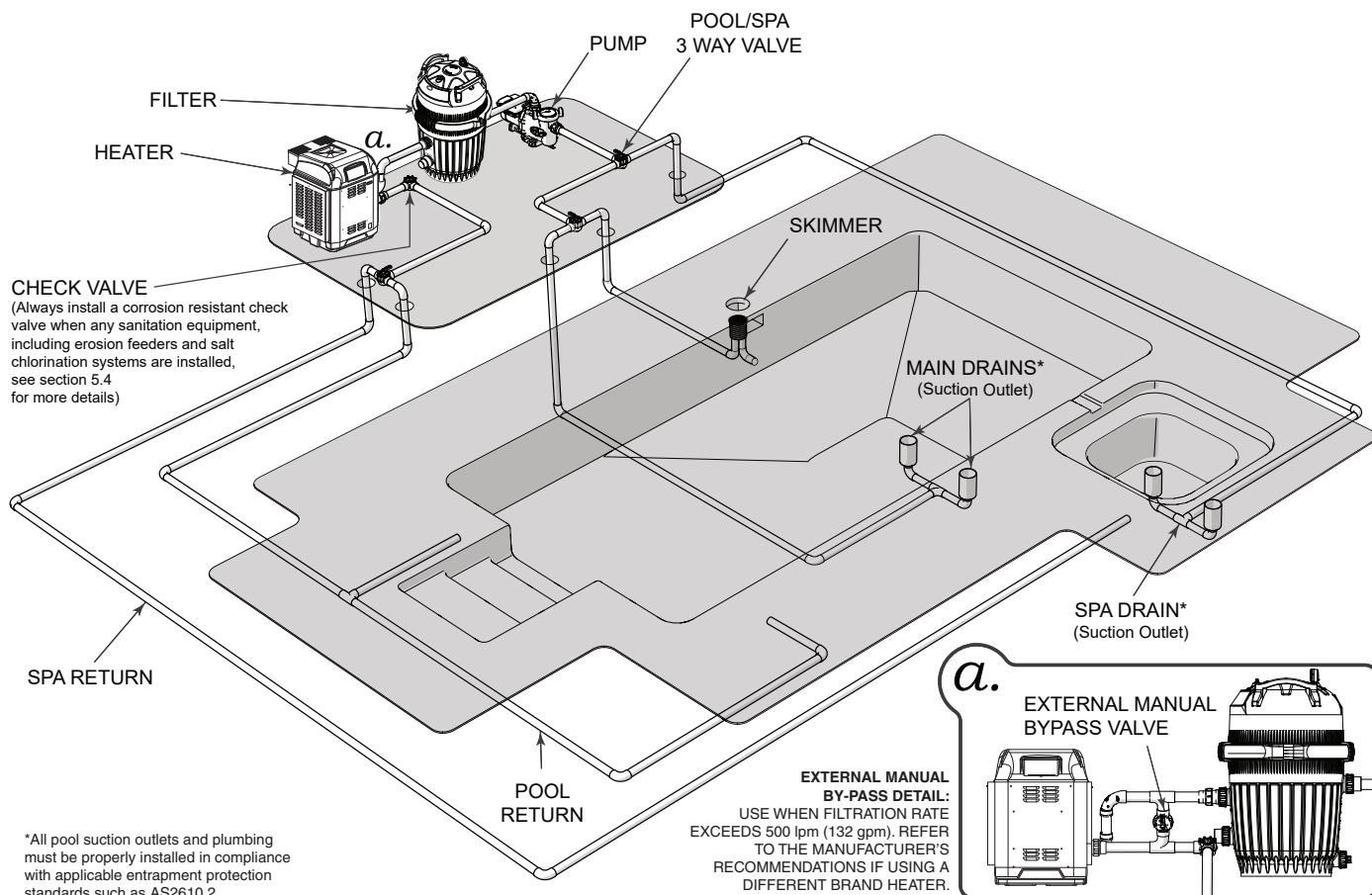
Figure 8. Typical Water Piping Configuration
