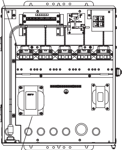
Power Center (with SCG option)
