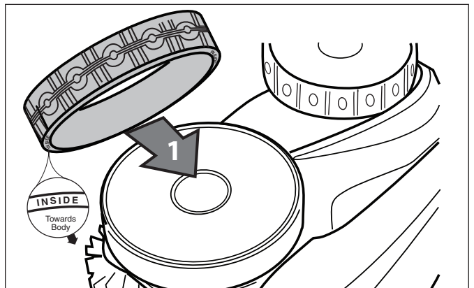
Figure 32. Tyre Replacement Orientation
