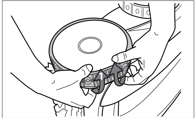
Figure 30. Pull the Old Tyre Over the Wheel
