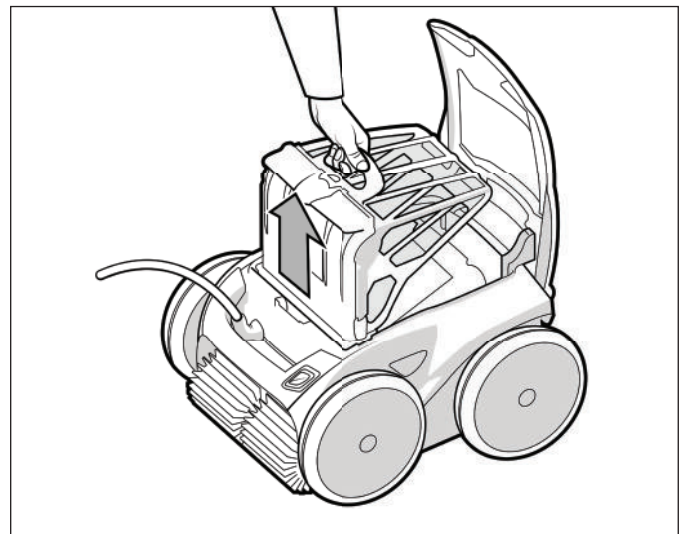
Figure 20. Remove the Filter Canisters
